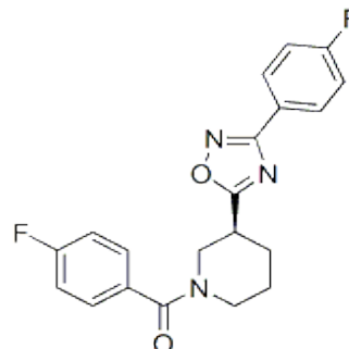
Chemical Structure
