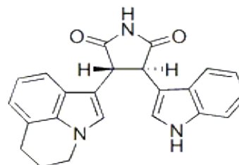
Chemical Structure
