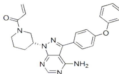
Chemical Structure
