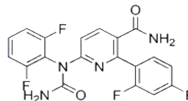
Chemical Structure
