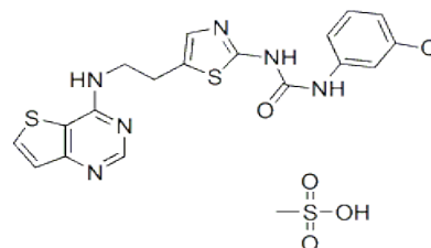
Chemical Structure
