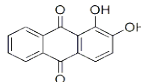
Chemical Structure
